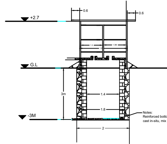
LATRINE BACK SECTION
