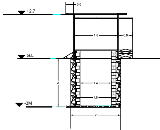
LATRINE SIDE SECTION
