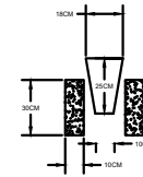
SQUAT SEAT AND FOOT REST DETAIL
