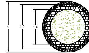
SECTAION. -3.M
